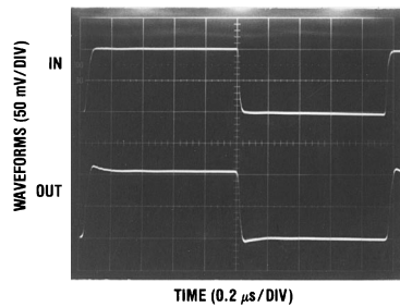
Noninverting Amp
