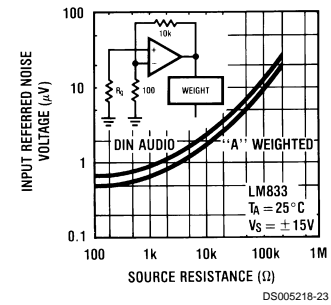
Input Referred Noise Voltage vs Source Resistance
